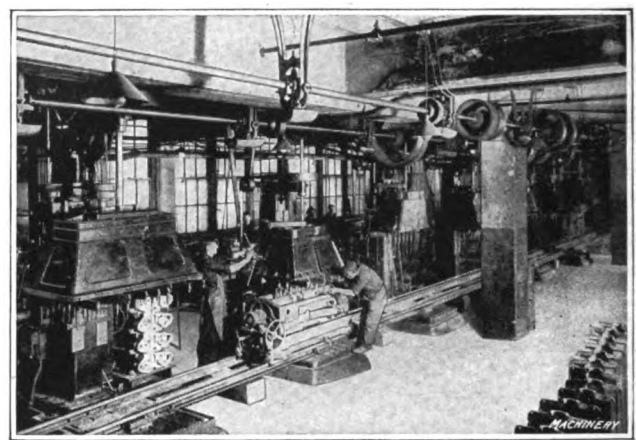
Fig. 12—At the Packard Motor Car Co.'s factory in Detroit, crank cases are drilled in jigs, which run on rails leading from machine to machine. These jigs are supported on trunnions and have index pins to enable all surfaces to be brought into the drilling position
